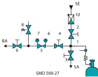
FLOW SCHEMATIC
