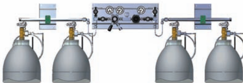
Installation example
